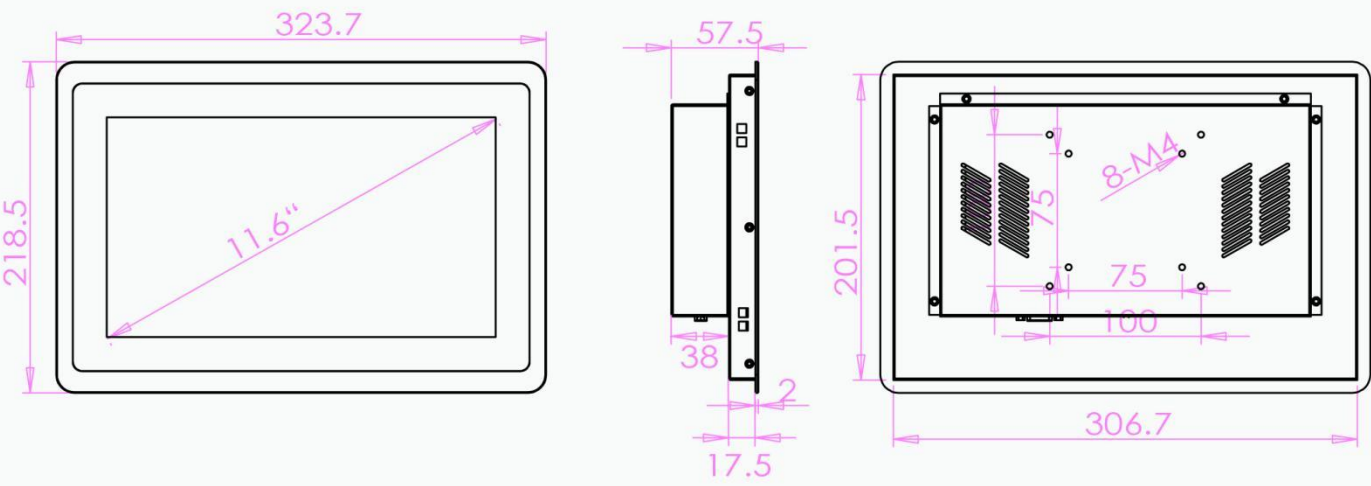
Front view
